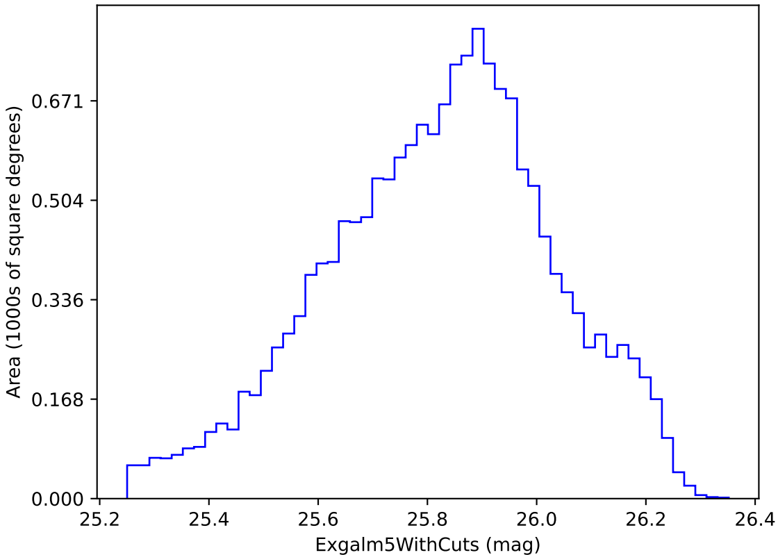
smc_lmc_v3.3_10yrs i band non-DD year 3: ExgalM5WithCuts
