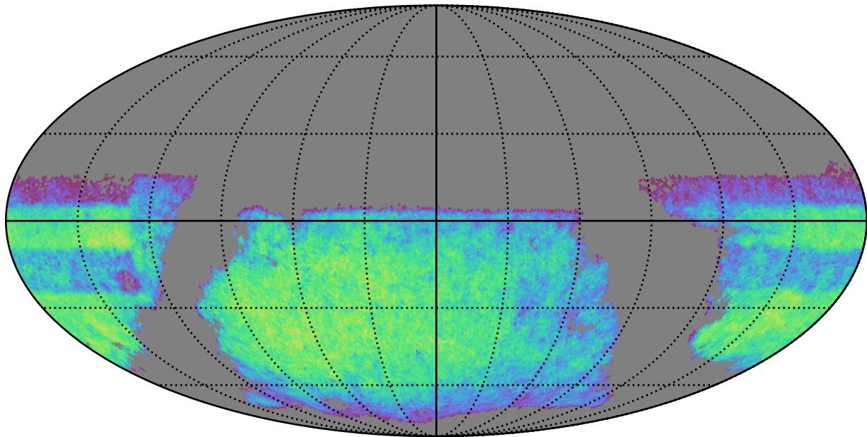
smc_lmc_v3.3_10yrs i band non-DD year 2: ExgalM5WithCuts
