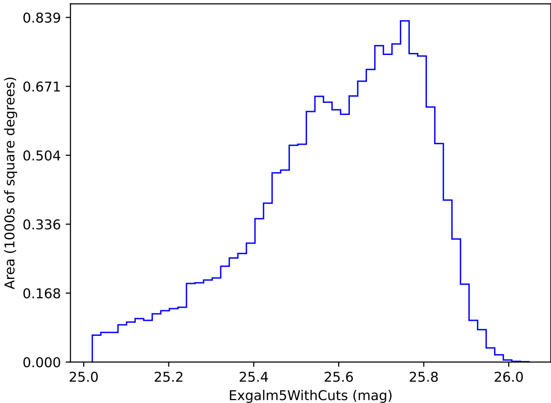
smc_lmc_v3.3_10yrs i band non-DD year 2: ExgalM5WithCuts
