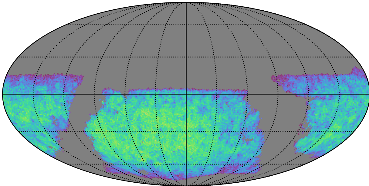
smc_lmc_v3.3_10yrs i band non-DD year 1: ExgalM5WithCuts
