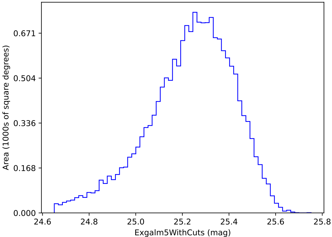
smc_lmc_v3.3_10yrs i band non-DD year 1: Exgal5WithCuts
