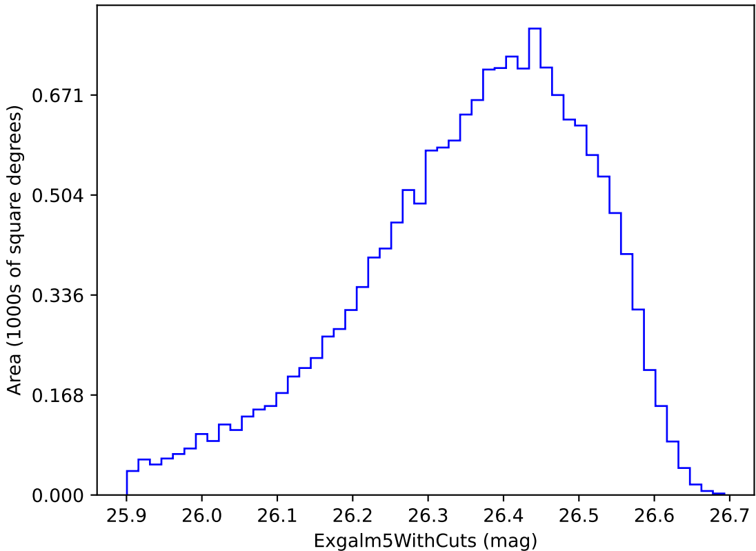
smc_lmc_v3.3_10yrs i band non-DD year 10: Exgal5WithCuts
