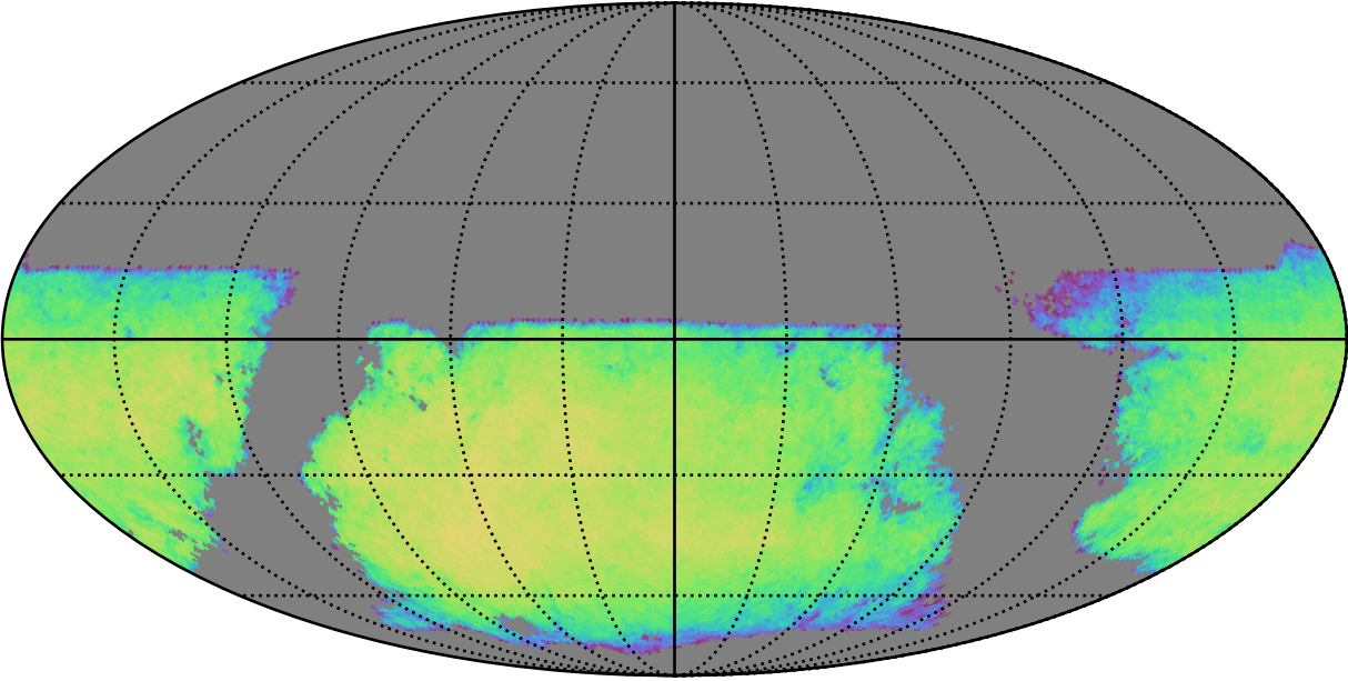
smc_lmc_v3.3_10yrs i band galaxies non-DD: DepthLimitedNumGalaxiesMetric
