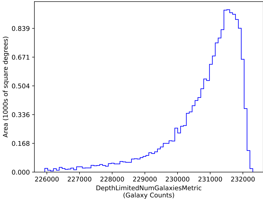
smc_lmc_v3.3_10yrs i band galaxies non-DD: DepthLimitedNumGalaxiesMetric
