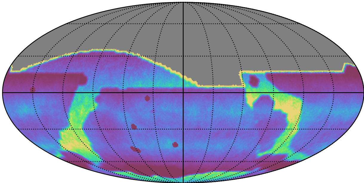
smc_lmc_v3.3_10yrs : DCRprecision
