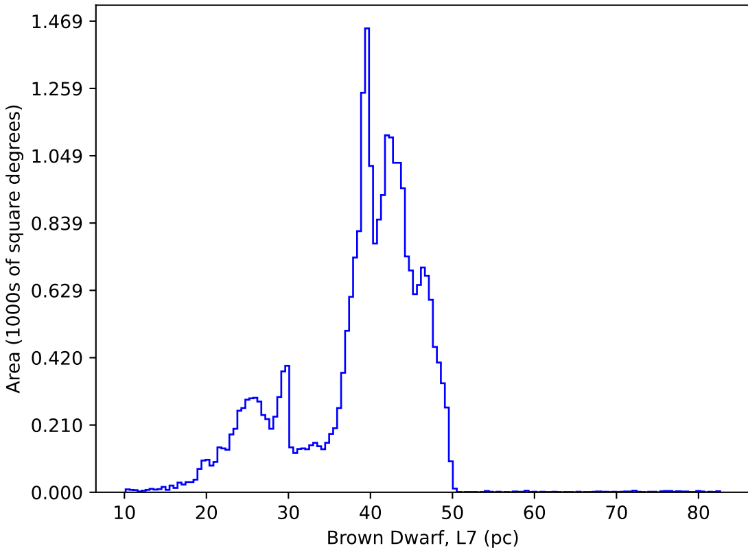
smc_lmc_v3.3_10yrs : Brown Dwarf, L7
