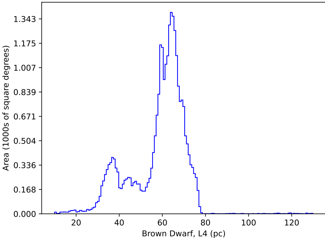
smc_lmc_v3.3_10yrs : Brown Dwarf, L4
