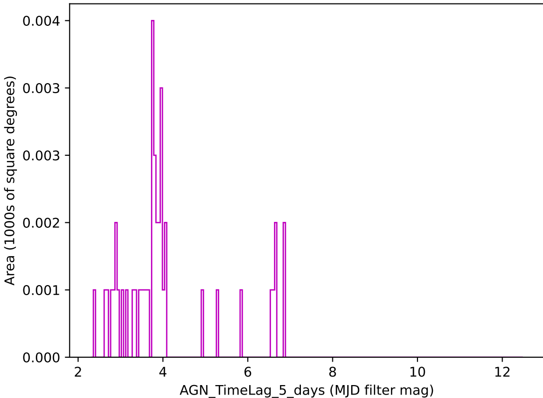
smc_lmc_v3.3_10yrs z band: AGN_TimeLag_5_days
