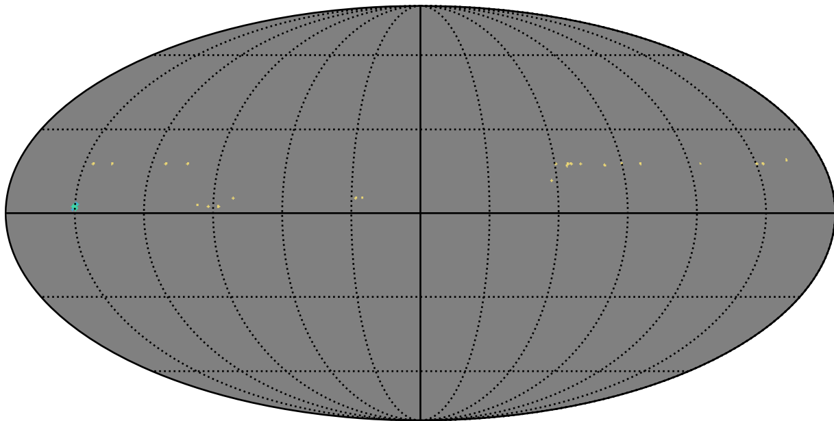
smc_lmc_v3.3_10yrs y band: AGN_TimeLag_5_days
