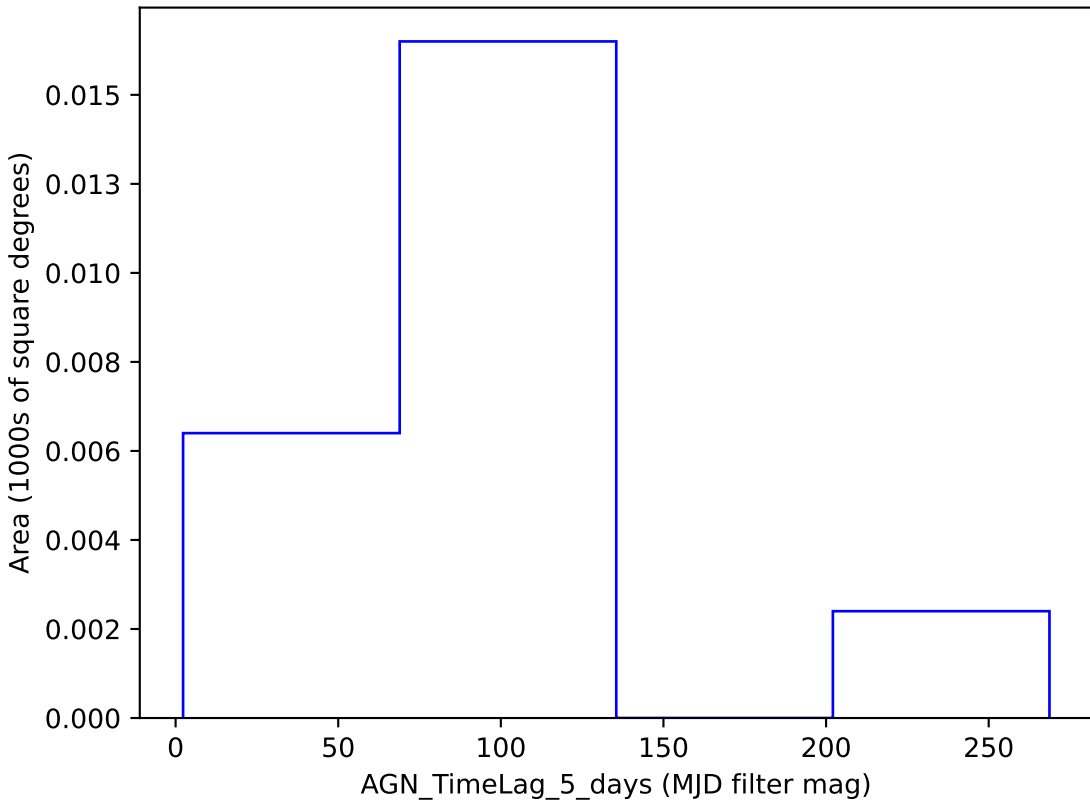
smc_lmc_v3.3_10yrs y band: AGN_TimeLag_5_days
