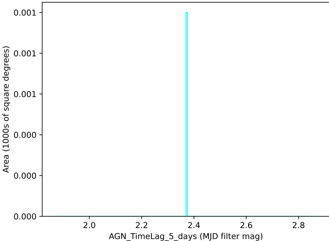
smc_lmc_v3.3_10yrs u band: AGN_TimeLag_5_days
