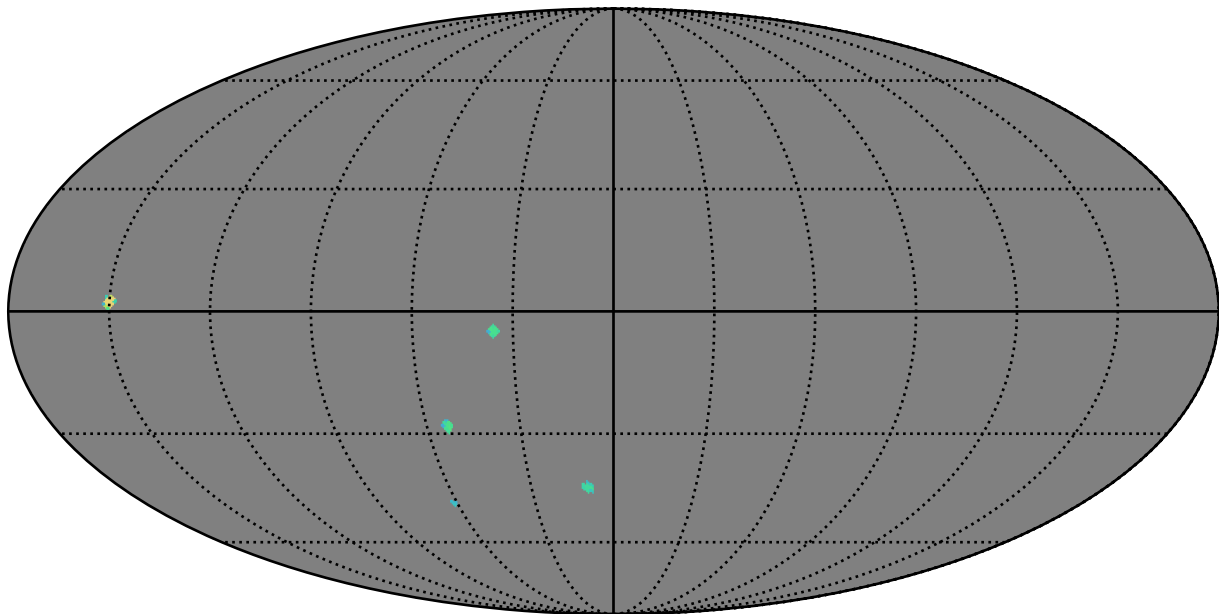
smc_lmc_v3.3_10yrs r band: AGN_TimeLag_5_days
