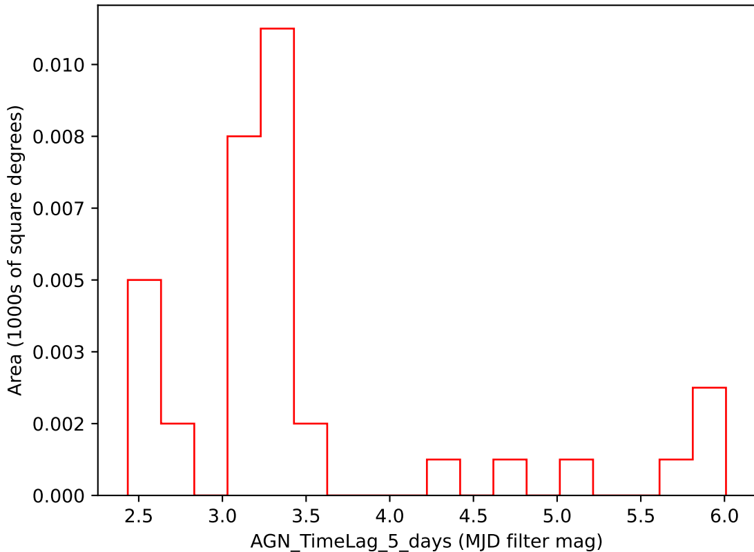
smc_lmc_v3.3_10yrs i band: AGN_TimeLag_5_days
