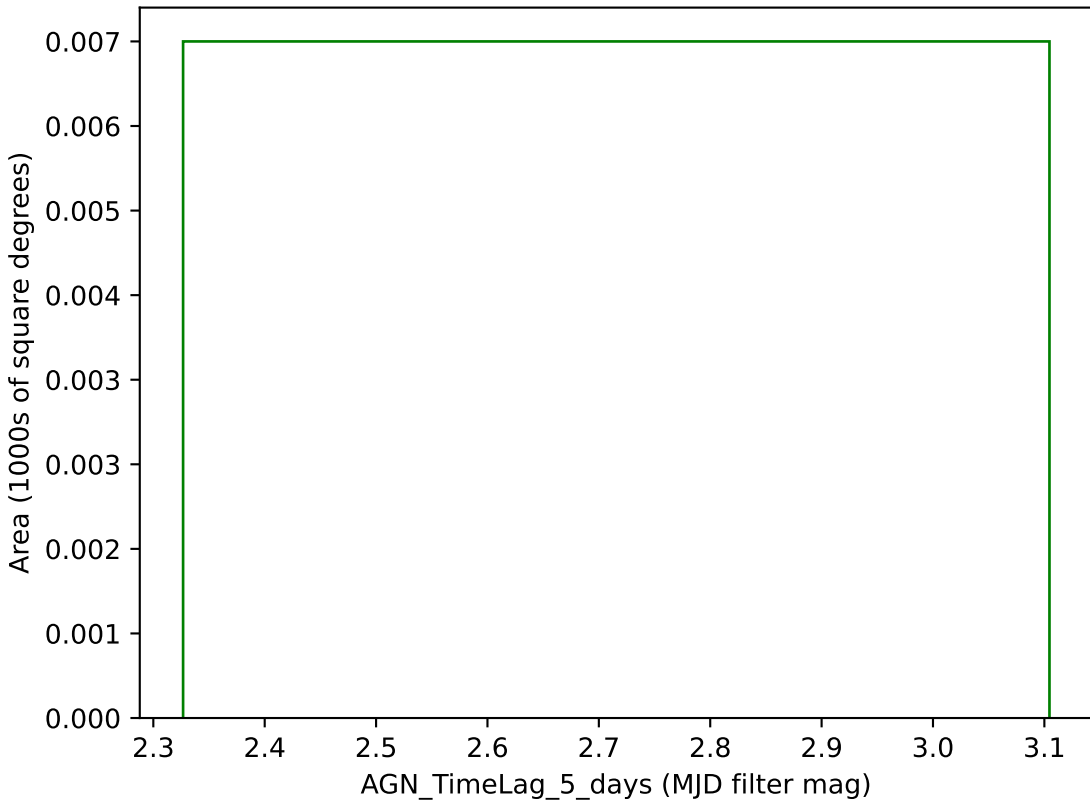
smc_lmc_v3.3_10yrs g band: AGN_TimeLag_5_days
