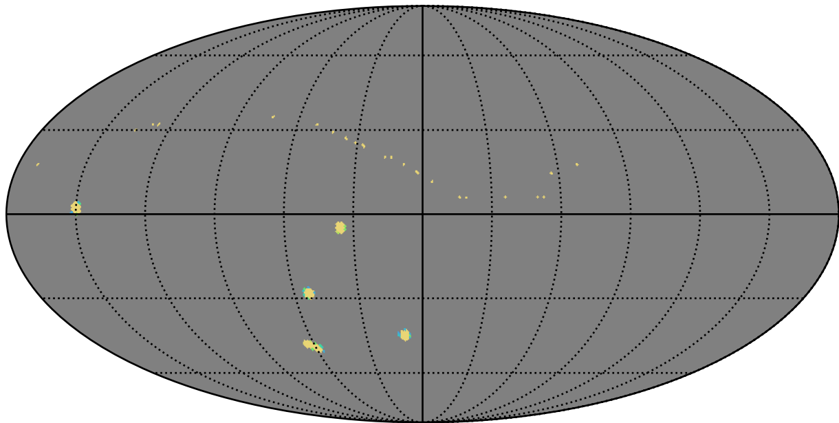
smc_lmc_v3.3_10yrs all bands: AGN_TimeLag_5_days
