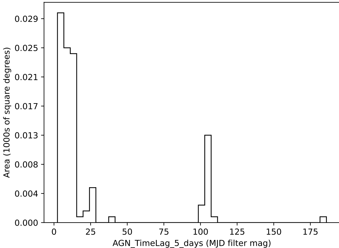
smc_lmc_v3.3_10yrs all bands: AGN_TimeLag_5_days
