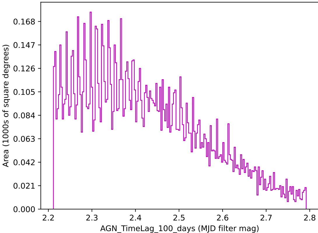
smc_lmc_v3.3_10yrs z band: AGN_TimeLag_100_days
