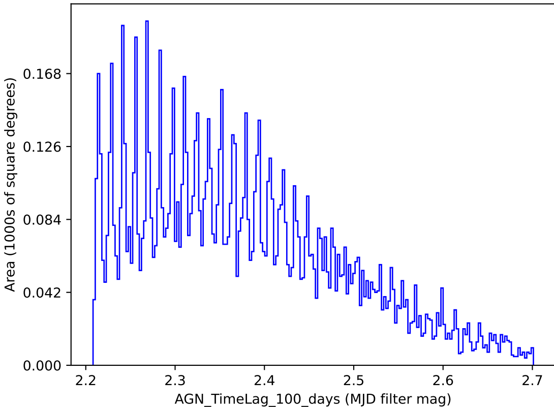
smc_lmc_v3.3_10yrs y band: AGN_TimeLag_100_days
