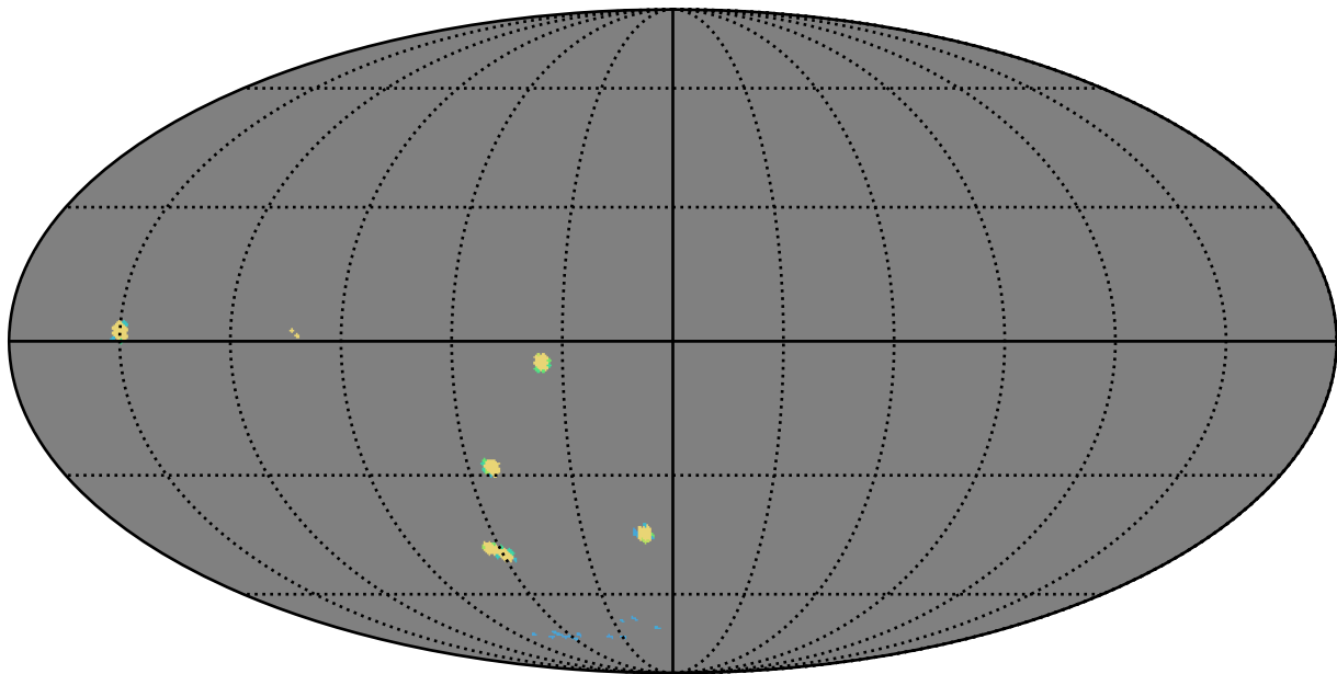
smc_lmc_v3.3_10yrs u band: AGN_TimeLag_100_days
