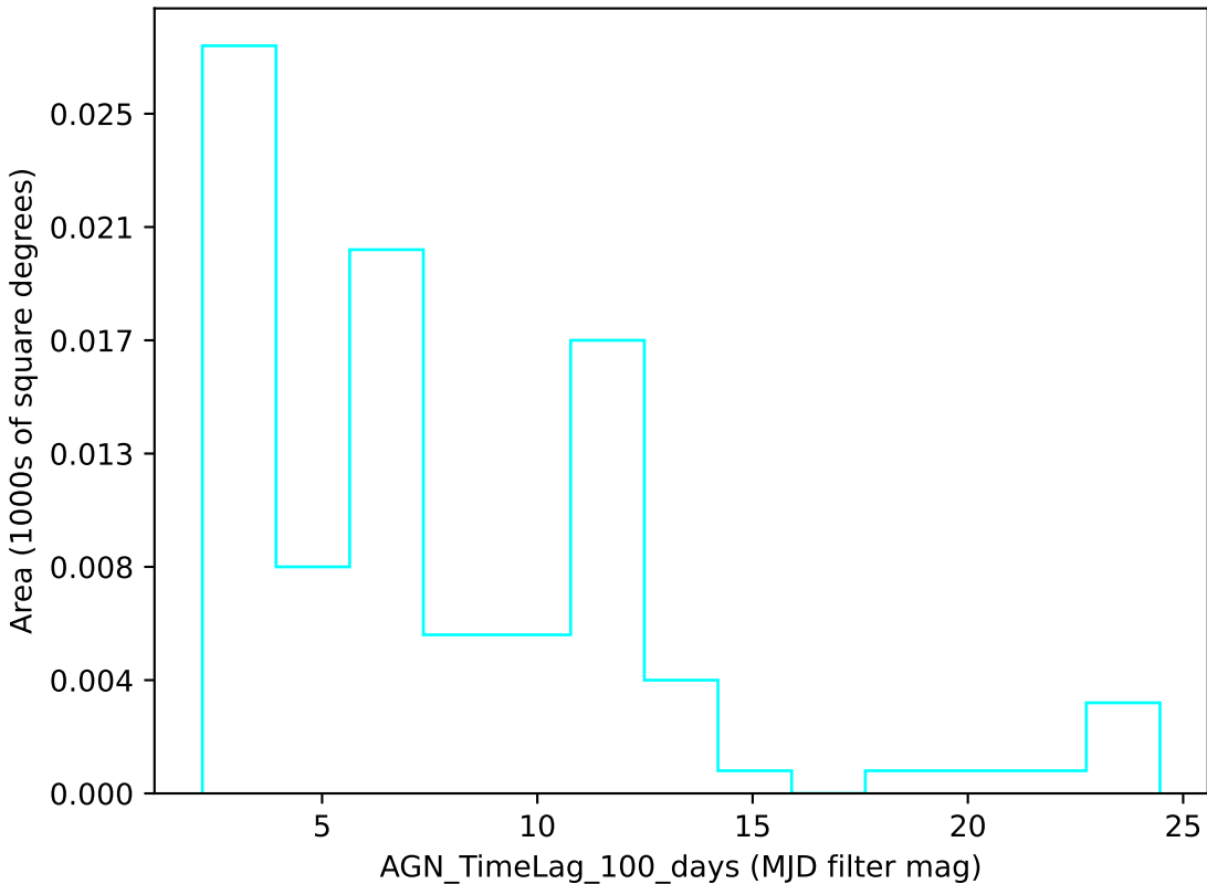
smc_lmc_v3.3_10yrs u band: AGN_TimeLag_100_days
