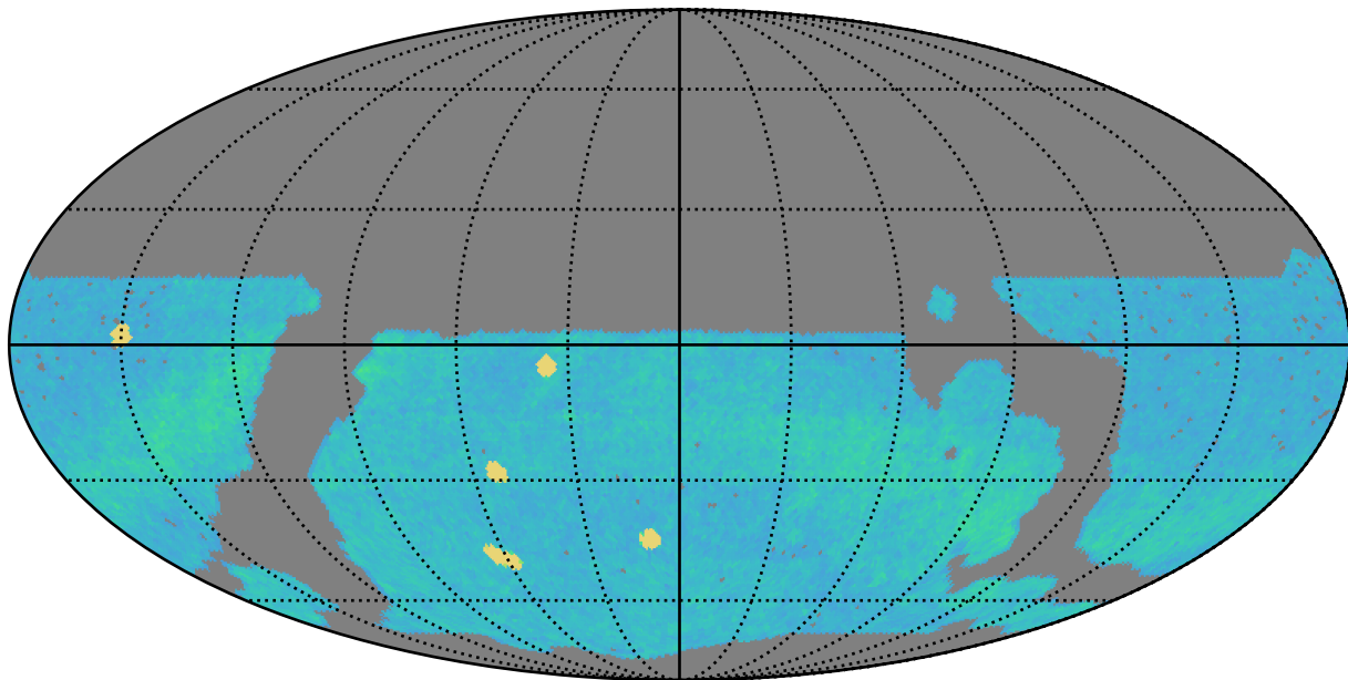
smc_lmc_v3.3_10yrs r band: AGN_TimeLag_100_days
