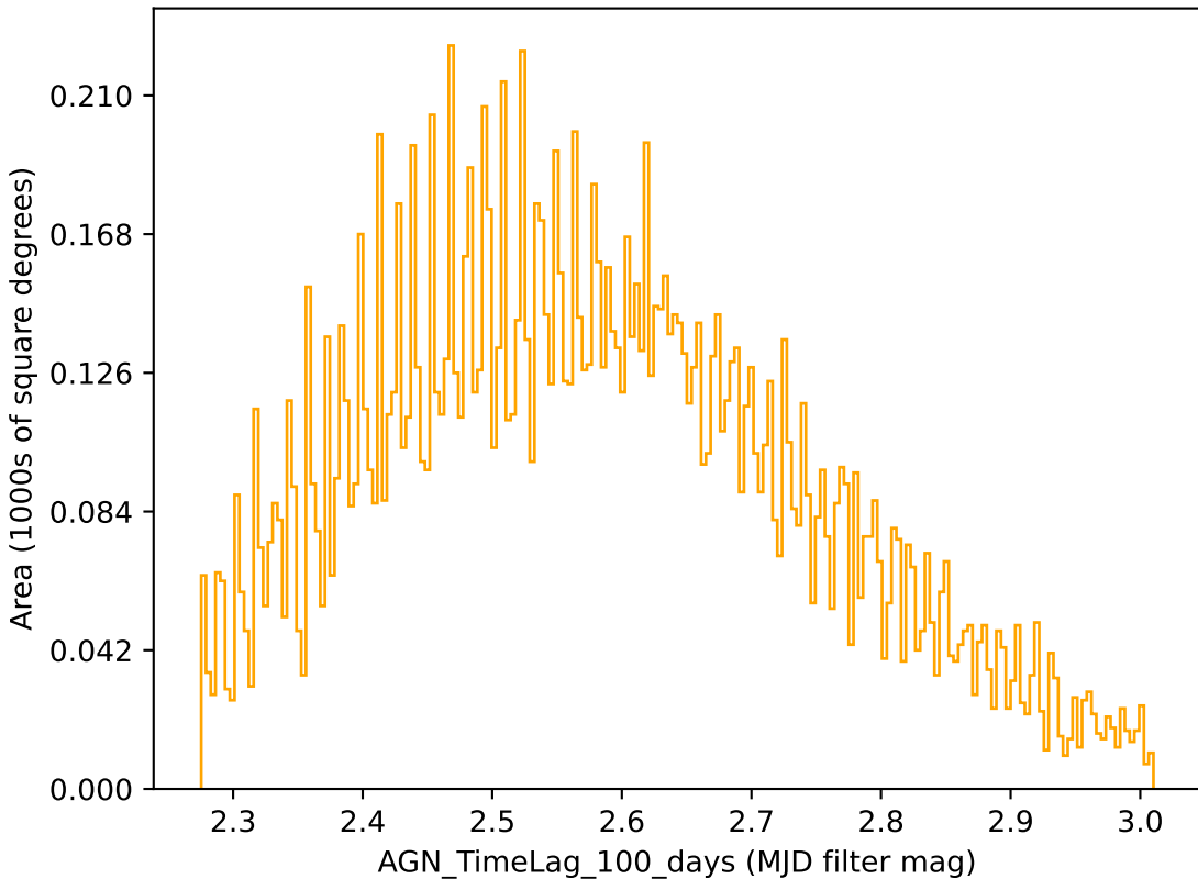
smc_lmc_v3.3_10yrs r band: AGN_TimeLag_100_days
