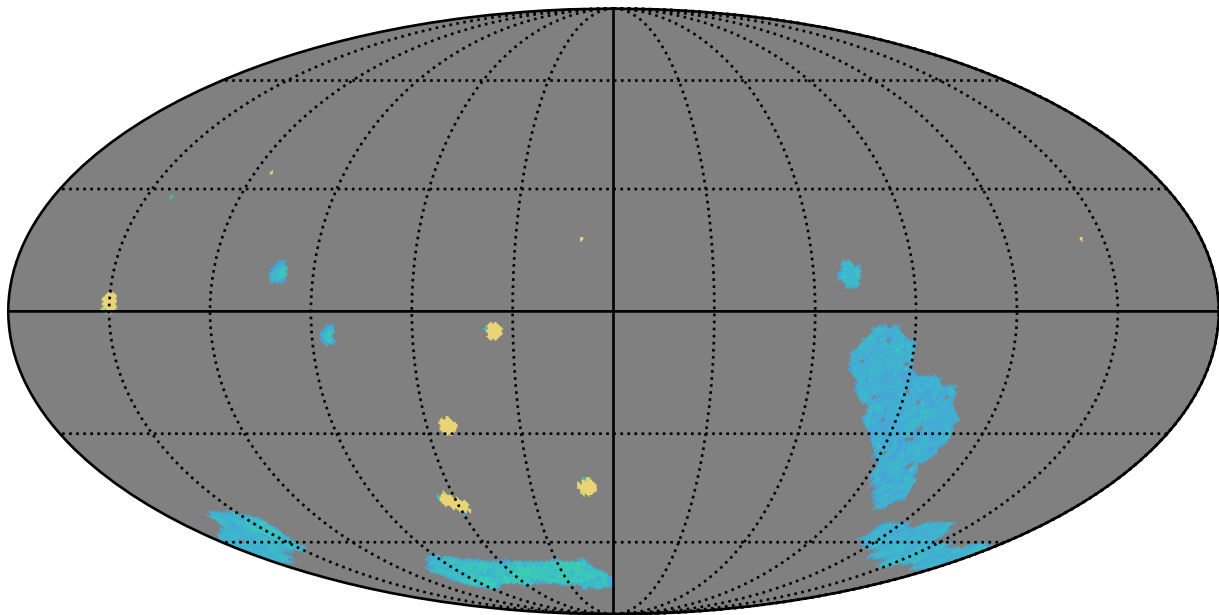
smc_lmc_v3.3_10yrs g band: AGN_TimeLag_100_days
