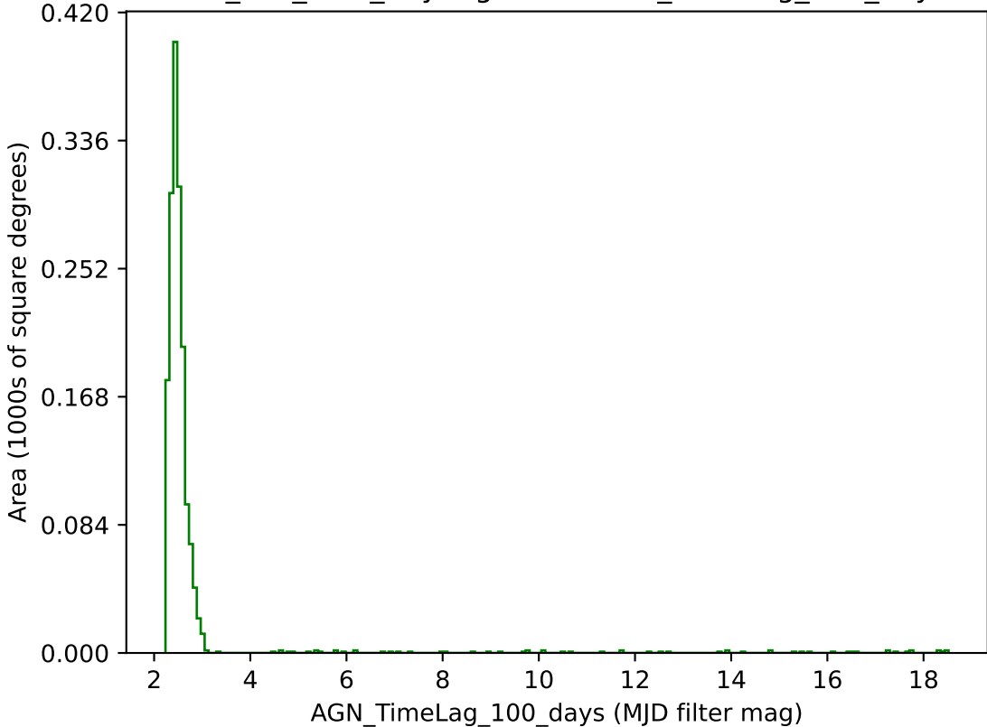
smc_lmc_v3.3_10yrs g band: AGN_TimeLag_100_days
