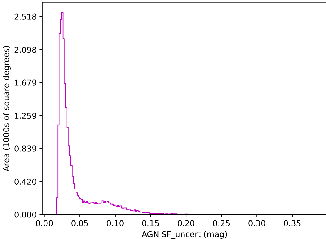
smc_lmc_v3.3_10yrs z band: AGN SF_uncert
