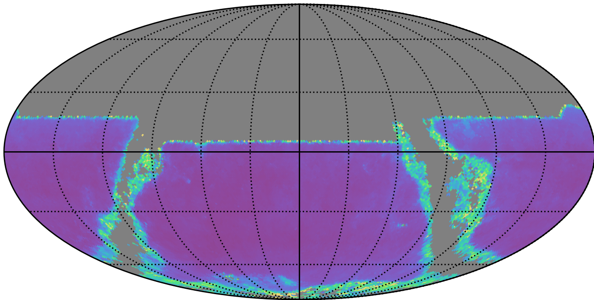
smc_lmc_v3.3_10yrs y band: AGN SF_uncert
