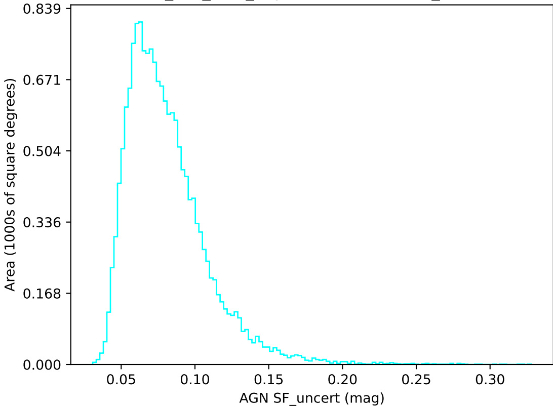
smc_lmc_v3.3_10yrs u band: AGN SF_uncert
