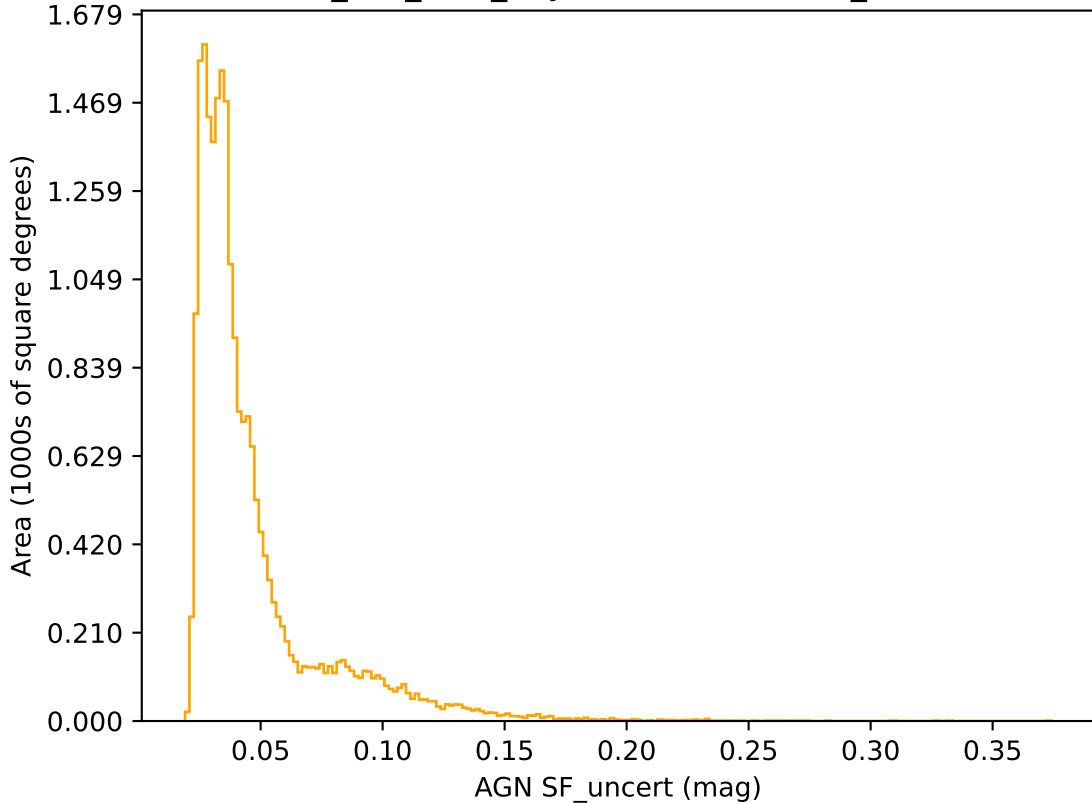
smc_lmc_v3.3_10yrs r band: AGN SF_uncert
