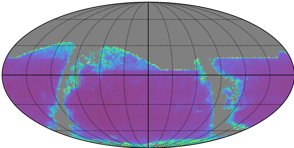
smc_lmc_v3.3_10yrs i band: AGN SF_uncert
