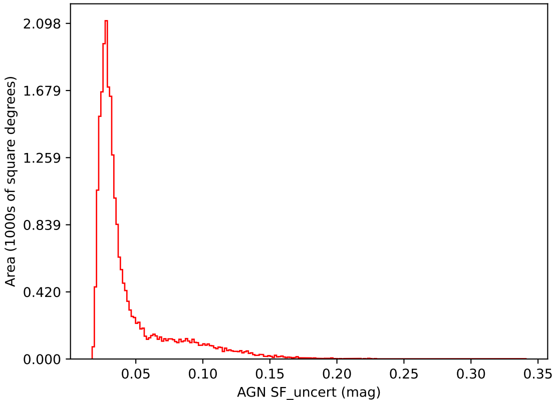
smc_lmc_v3.3_10yrs i band: AGN SF_uncert
