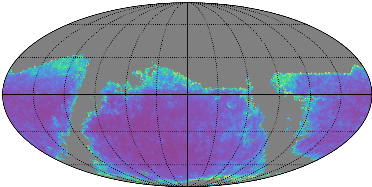
smc_lmc_v3.3_10yrs g band: AGN SF_uncert
