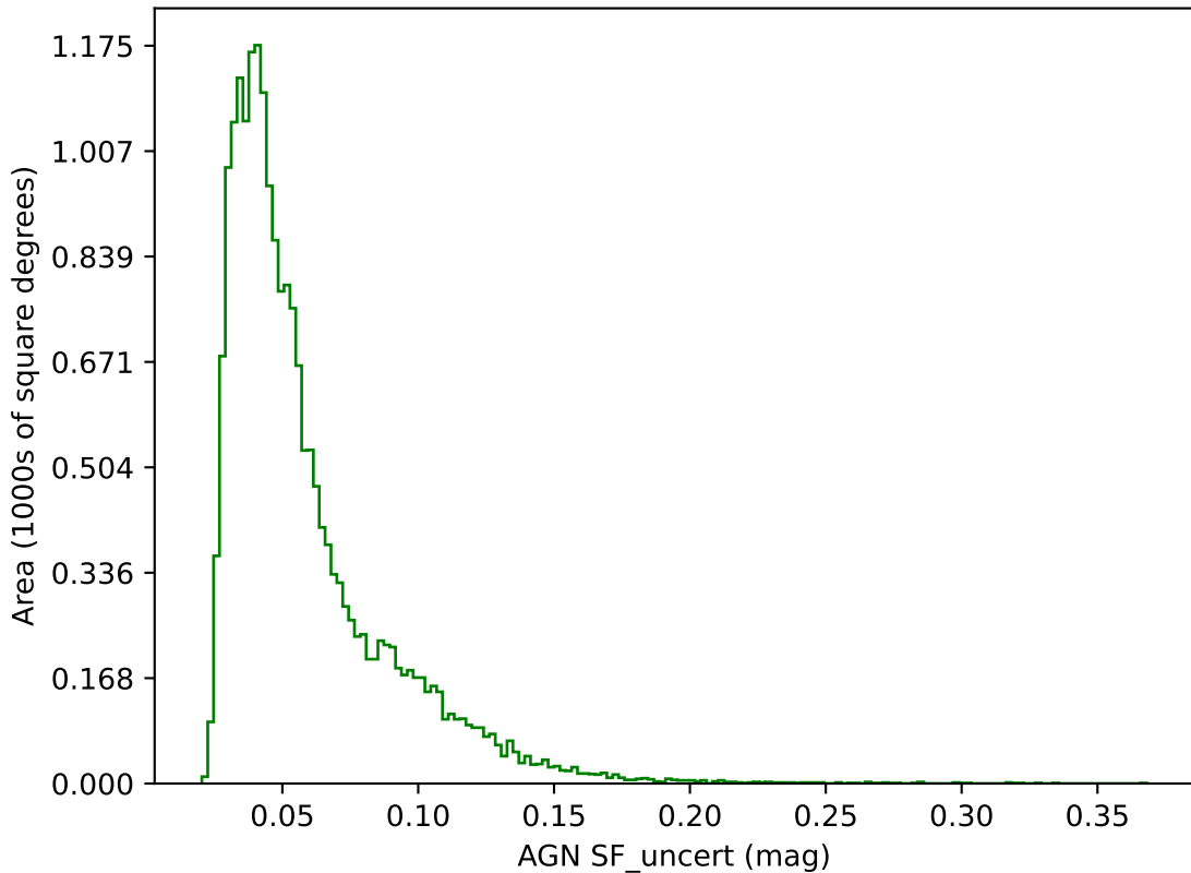
smc_lmc_v3.3_10yrs g band: AGN SF_uncert
