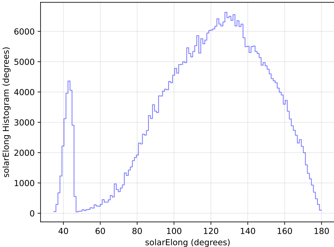
smc_lmc_v3.3_10yrs WFD z band: solarElong Histogram
