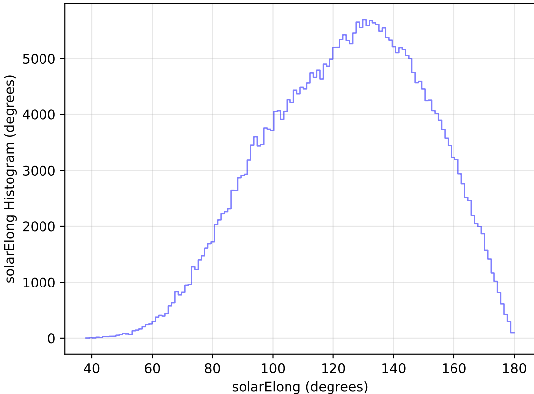
smc_lmc_v3.3_10yrs WFD y band: solarElong Histogram
