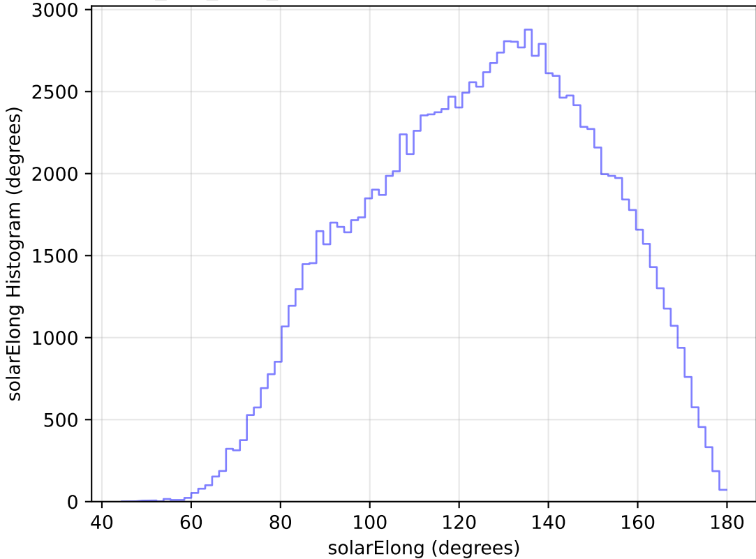
smc_lmc_v3.3_10yrs WFD u band: solarElong Histogram
