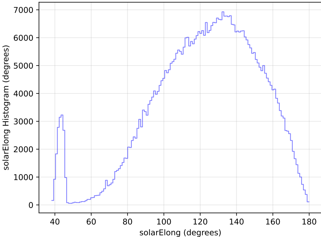
smc_lmc_v3.3_10yrs WFD r band: solarElong Histogram
