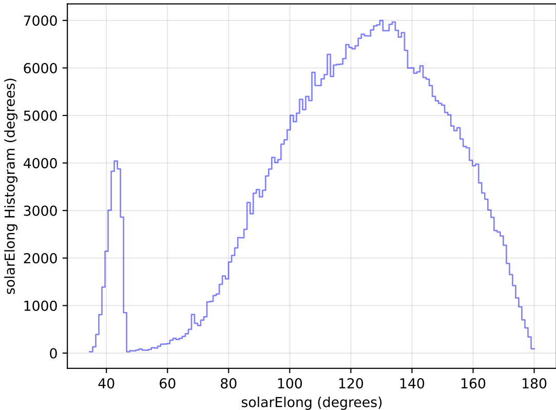
smc_lmc_v3.3_10yrs WFD i band: solarElong Histogram
