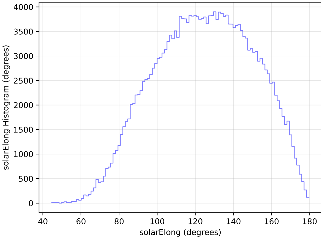
smc_lmc_v3.3_10yrs WFD g band: solarElong Histogram
