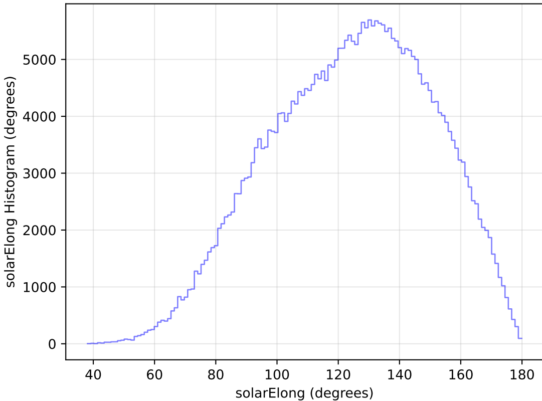
smc_lmc_v3.3_10yrs All sky y band: solarElong Histogram
