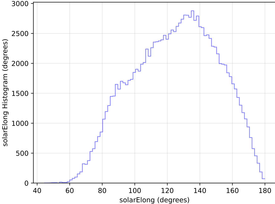
smc_lmc_v3.3_10yrs All sky u band: solarElong Histogram
