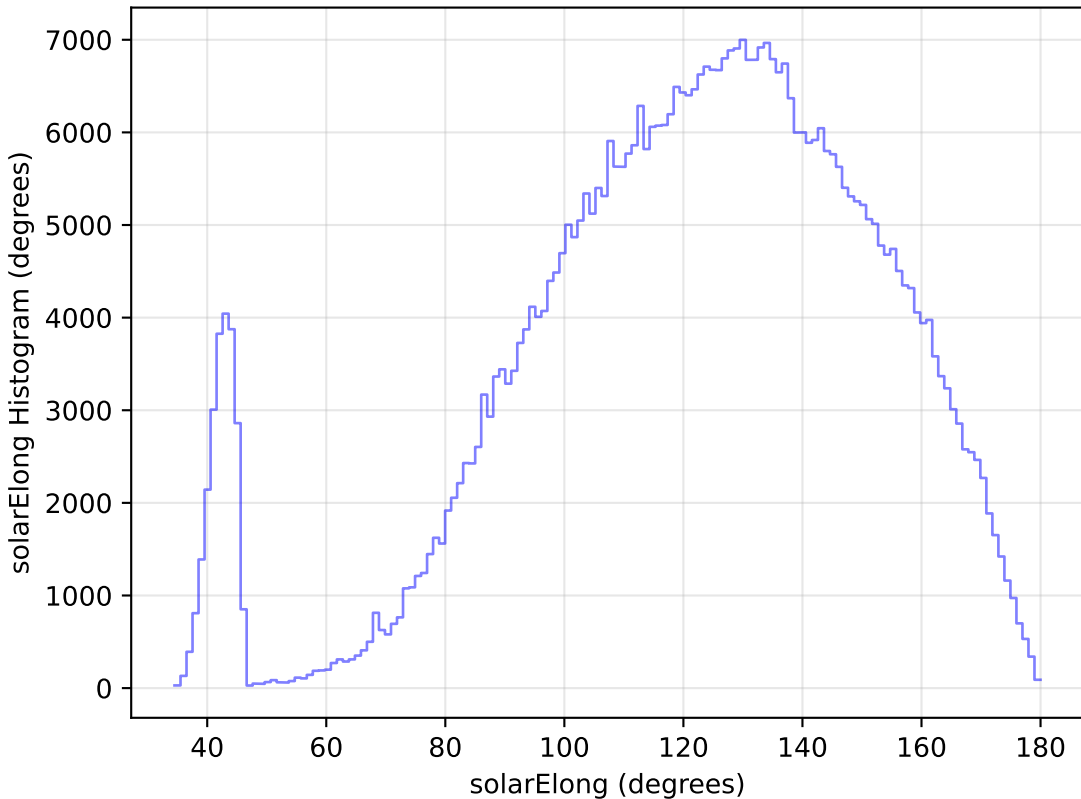
smc_lmc_v3.3_10yrs All sky i band: solarElong Histogram
