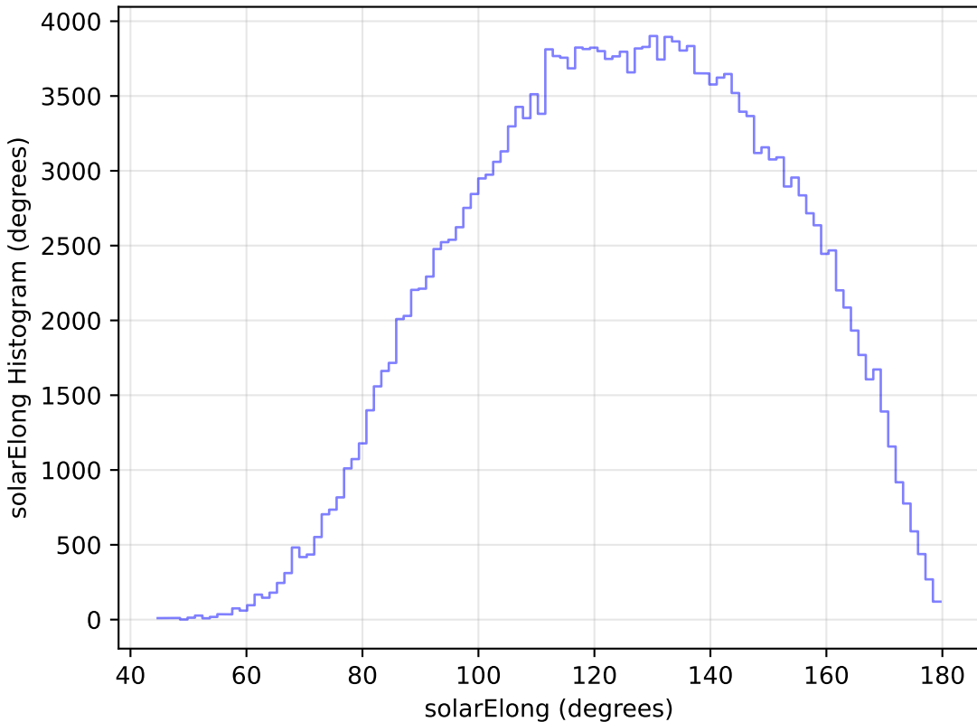
smc_lmc_v3.3_10yrs All sky g band: solarElong Histogram
