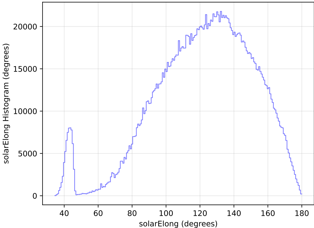
smc_lmc_v3.3_10yrs All sky all bands: solarElong Histogram
