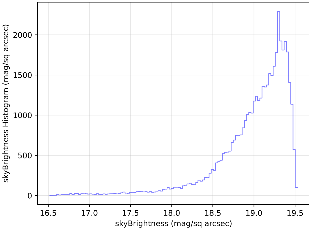
smc_lmc_v3.3_10yrs Yr 1 z band: skyBrightness Histogram
