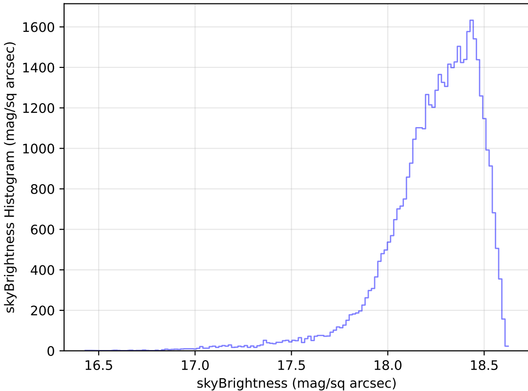
smc_lmc_v3.3_10yrs Yr 1 y band: skyBrightness Histogram
