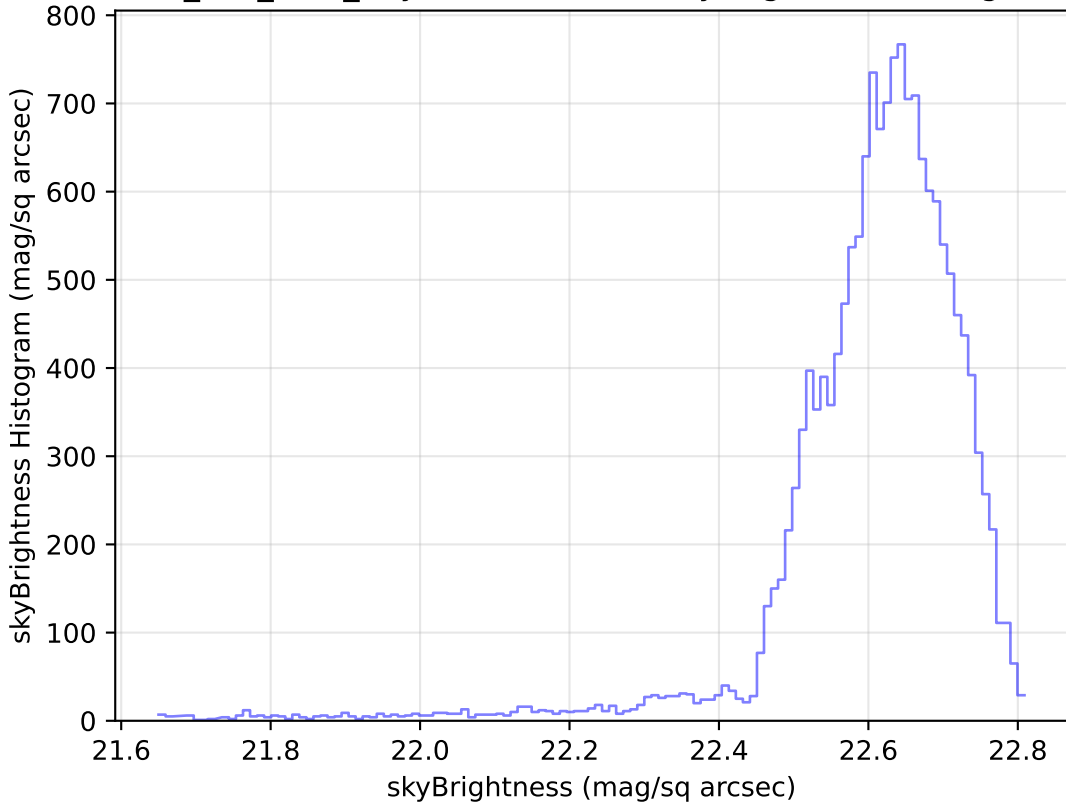
smc_lmc_v3.3_10yrs Yr 1 u band: skyBrightness Histogram
